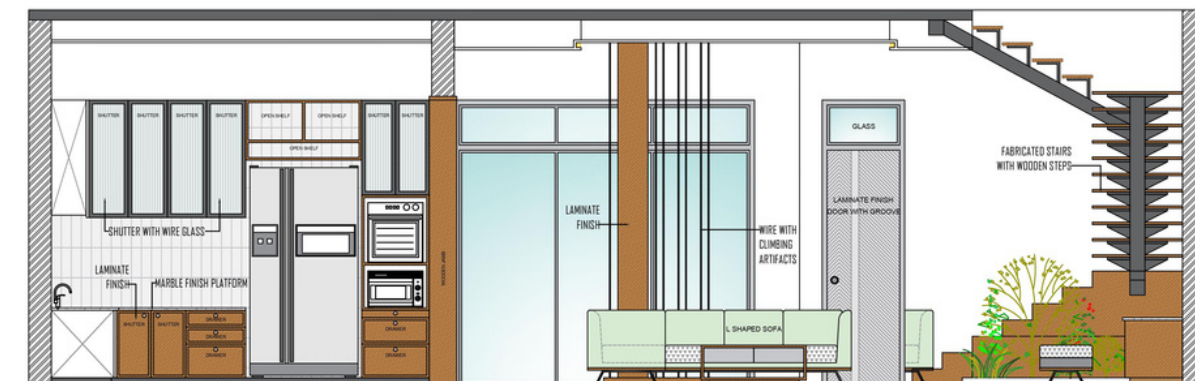
ELEVATION-D
