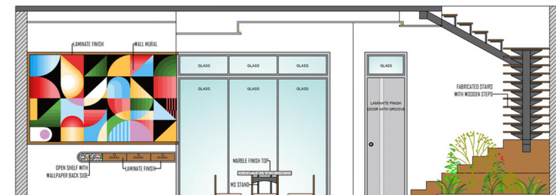
ELEVATION-D'
